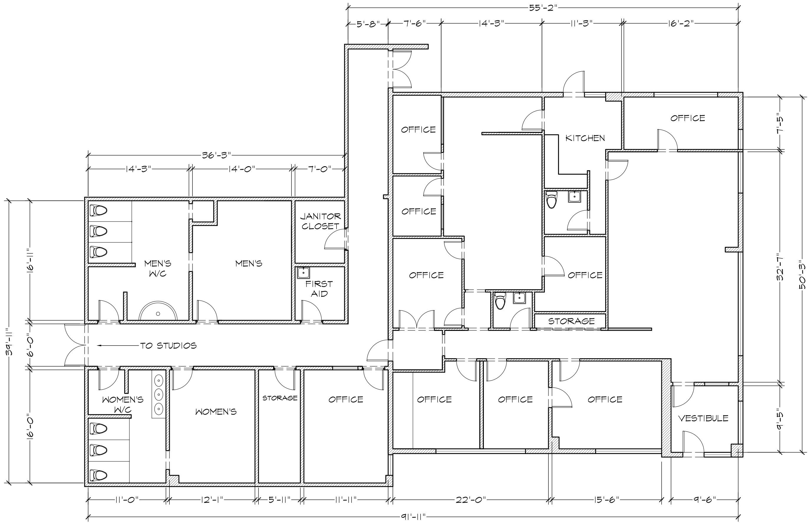
PLAN OF 40 BUTTERICK RD., OFFICE SPACE- MAIN FLOOR SCALE: 1/8" = 1'-0"
