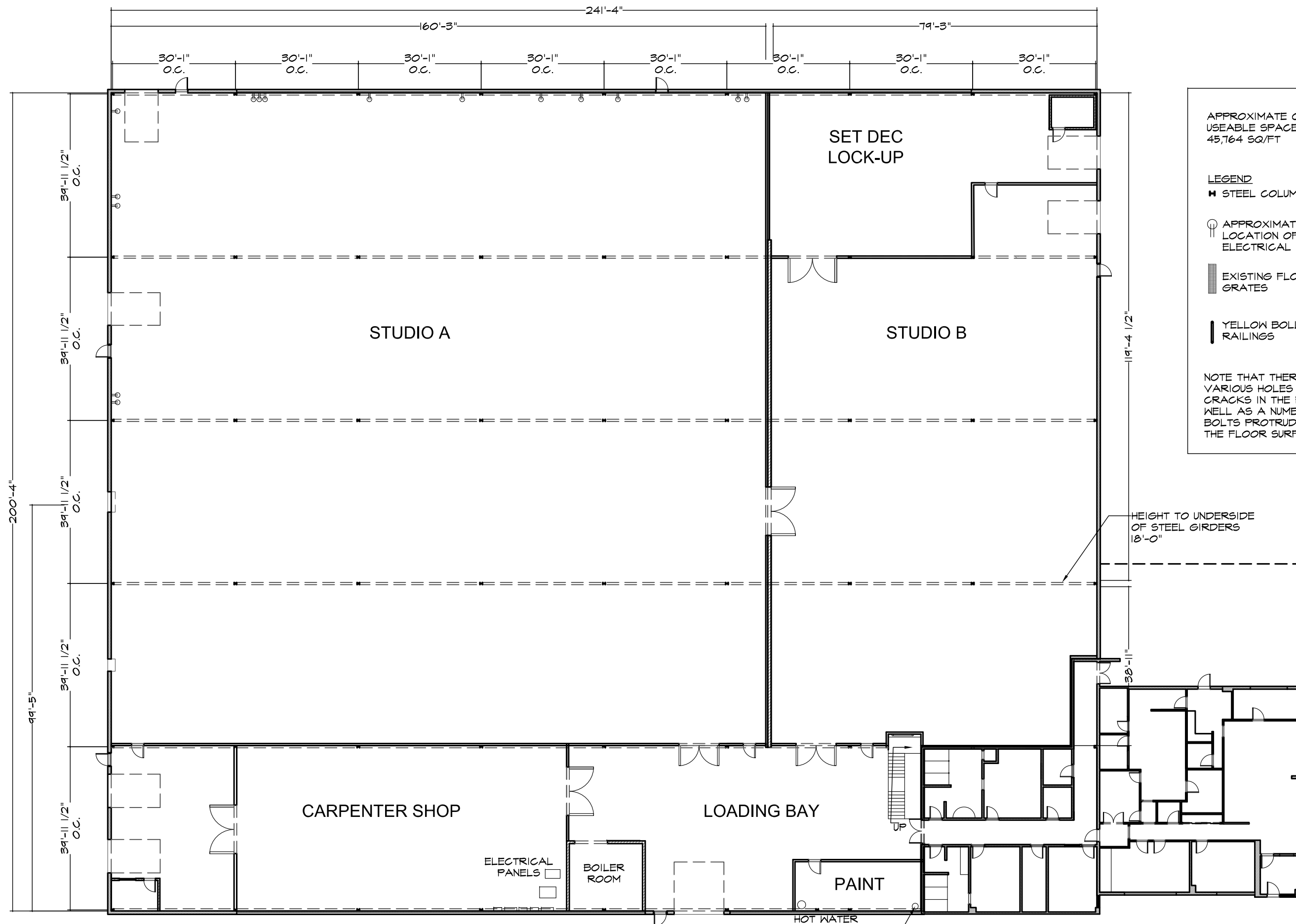
PLAN OF 40 BUTTERICK RD., STUDIO SPACE
